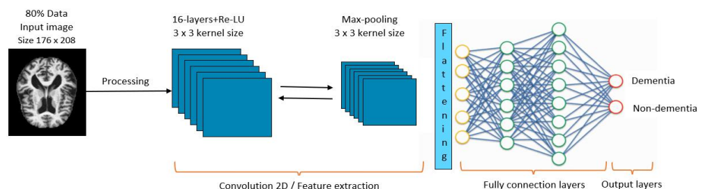
Figure 4. Proposed Convolution Neural Network model
